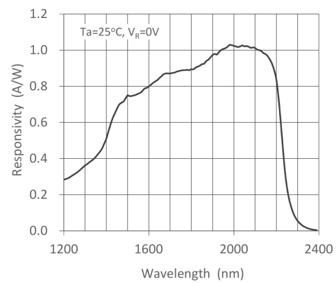
Spectral Responsivity
