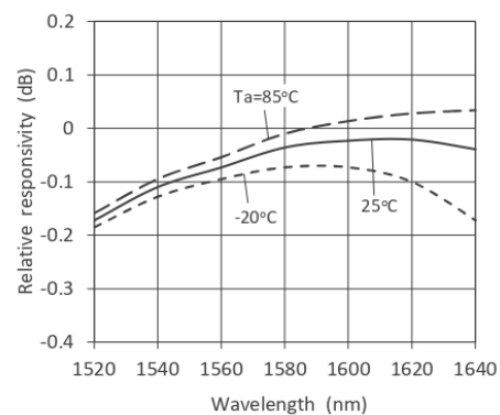
Uniformity of Spectral Responsivity
