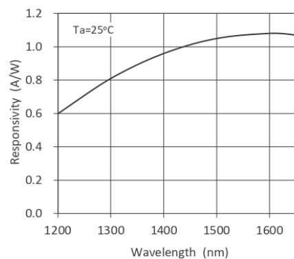
Spectral Responsivity
