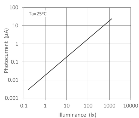
Photocurrent - Illuminance
