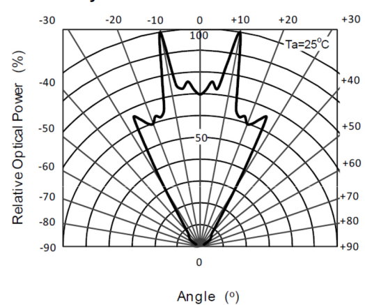
Directivity
