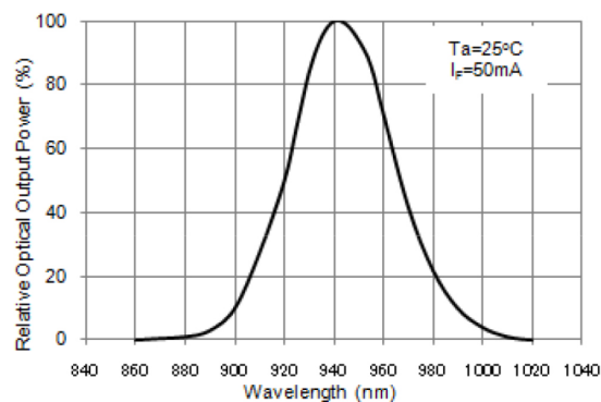
Spectral Distribution
