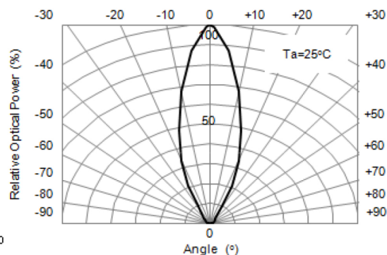
Directivity
